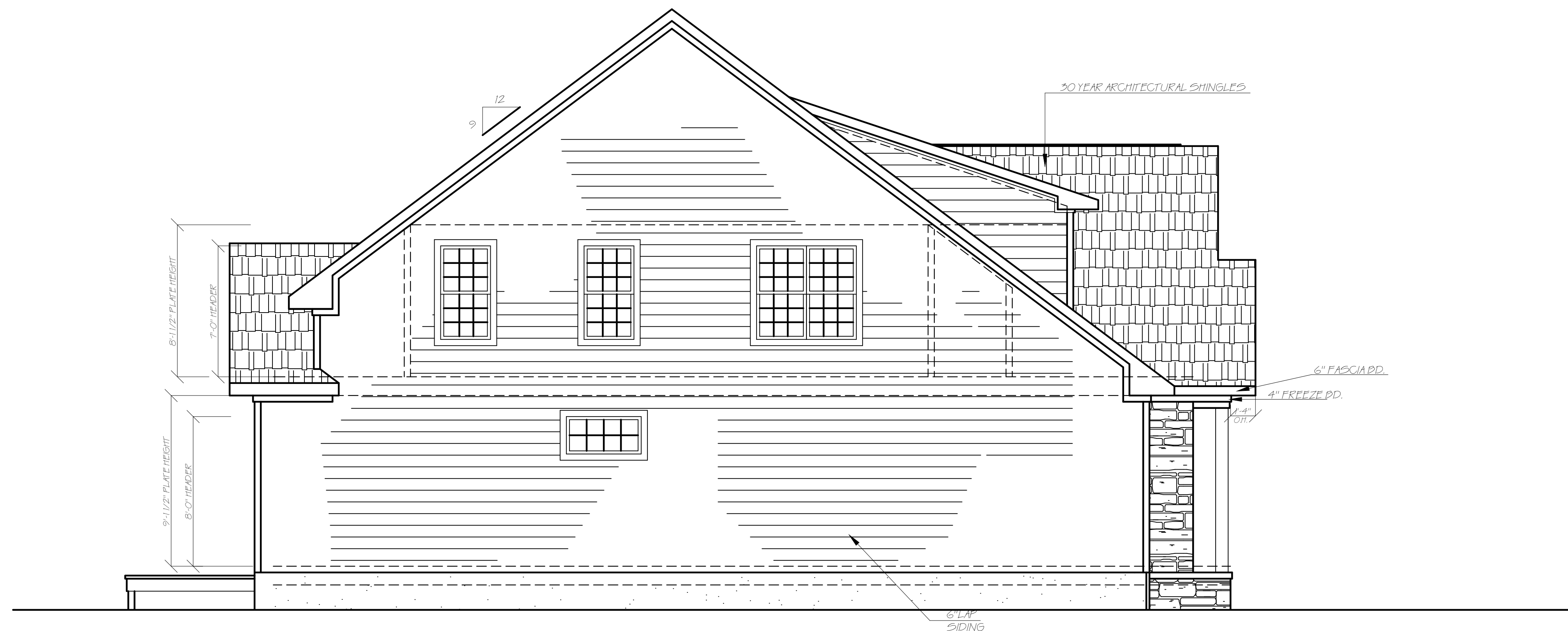
LEFT ELEVATION
